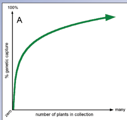
Graph A: The conservationist’s curve: graph of collection size vs. allele capture.
